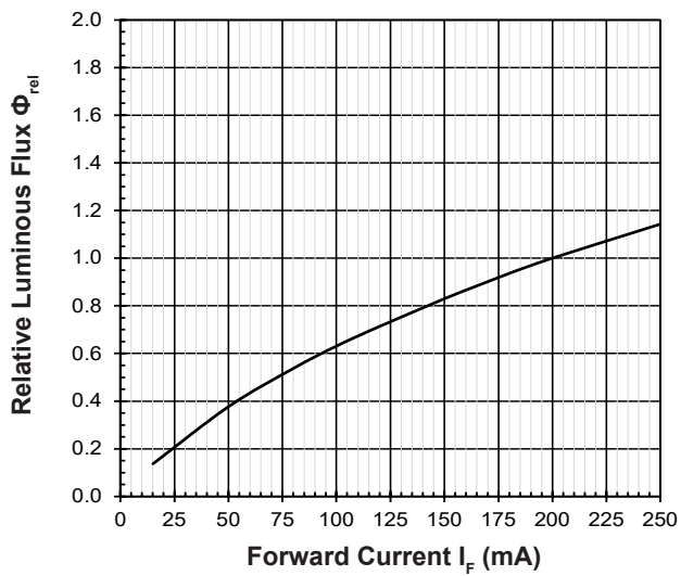
Relative Luminous Flux Vs Forward Current \Phi_V/\Phi_V(200\text{mA}) = f(I_F); T_j = 25^\circ\text{C} (True Green)
