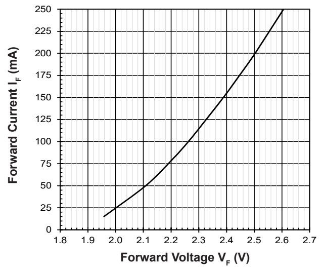
Forward Current Vs Forward Voltage I_F = f(V_F); T_j = 25^\circ\text{C} (Red)
