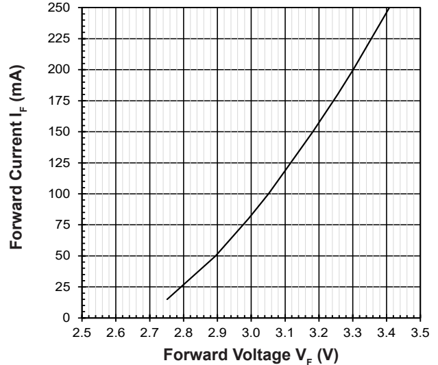
Forward Current Vs Forward Voltage I_F = f(V_F); T_j = 25^\circ\text{C} (Blue)
