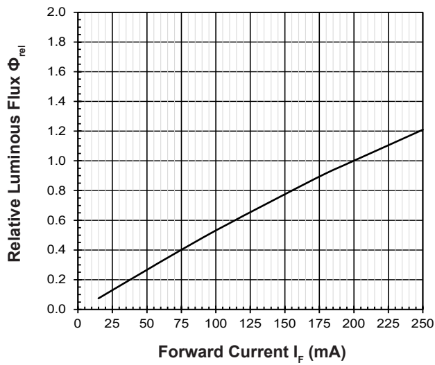
Relative Luminous Flux Vs Forward Current \Phi_V/\Phi_V(200\text{mA}) = f(I_F); T_j = 25^\circ\text{C} (Red)
