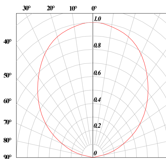
Radiation Pattern
