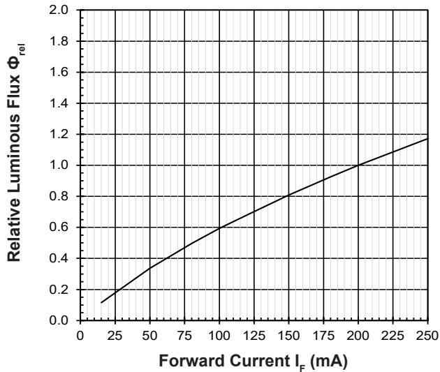
Relative Luminous Flux Vs Forward Current \Phi_V/\Phi_V(200\text{mA}) = f(I_F); T_j = 25^\circ\text{C} (Blue)
