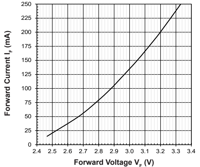
Forward Current Vs Forward Voltage I_F = f(V_F); T_j = 25^\circ\text{C} (True Green)
