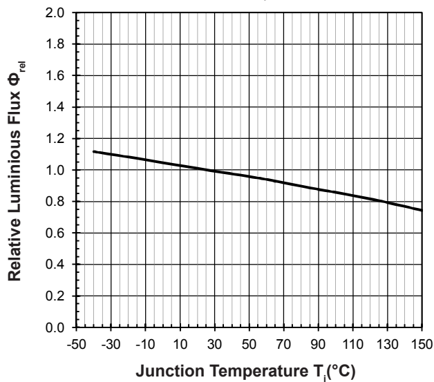
Relative Luminous Flux Vs Junction Temperature Appx. 4.1
