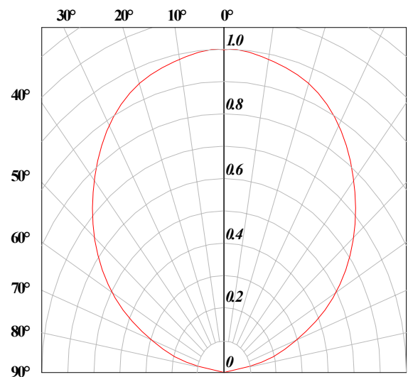
Radiation Pattern
