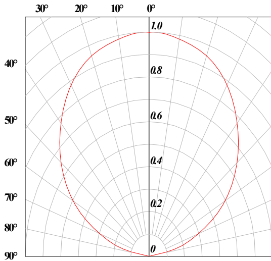
Radiation Pattern
