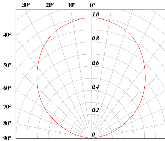
Radiation Pattern
