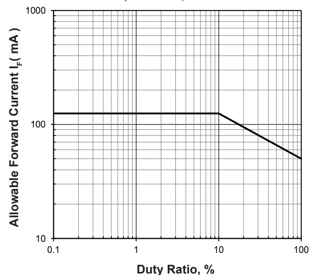
Allowable Forward Current Vs Duty Ratio
