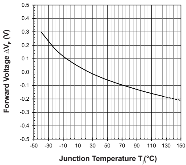
Forward Voltage Vs Junction Temperature Appx. 4.1
