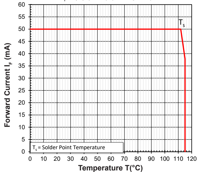
Maximum Current Vs Temperature (Red) (1 chip on) I_F = f(T)
