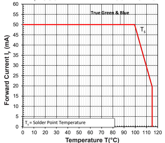
Maximum Current Vs Temperature (Blue & True Green) (1 chip on) I_F = f(T)
